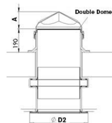
Figure A1: Schematic representations of the different models of Chatron Solar Light Tube.
