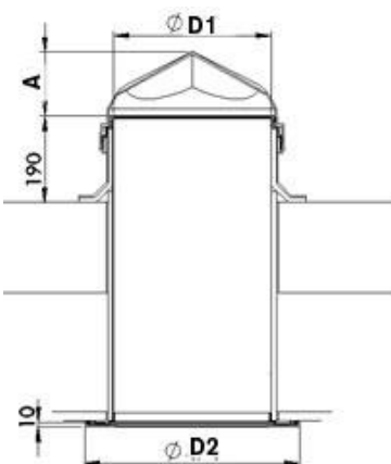
Figure A1: Schematic representations of the different models of Chatron Solar Light Tube.
